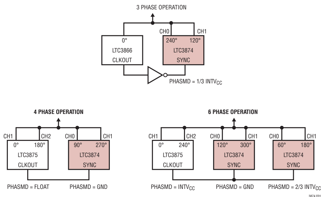
Figure 1. Multiphase Operation
