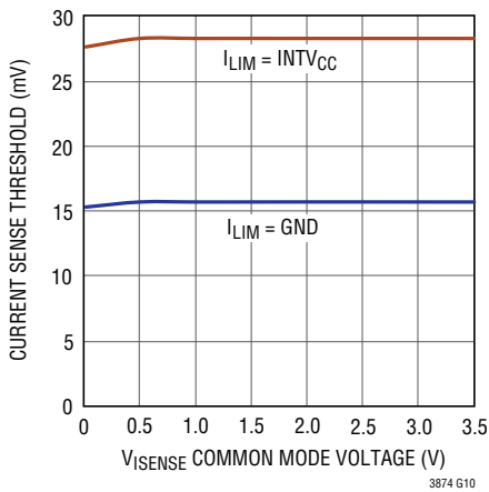
Maximum Current Sense Threshold vs Common Mode Voltage ( \text{LOWDCR} = \text{INTV}_{\text{CC}} , V_{\text{ITH}} = 2.18\text{V} )
