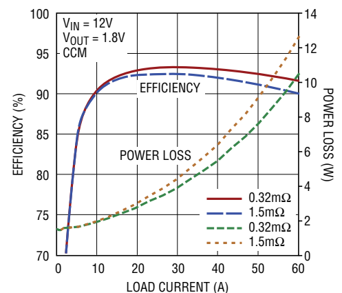
Dual Phase Efficiency and Power Loss vs Output Current, Sub-Milliohm DCR vs Traditional DCB
