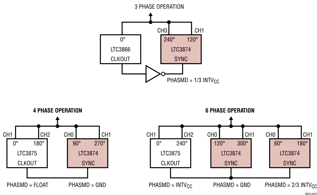
Figure 1. Multiphase Operation
