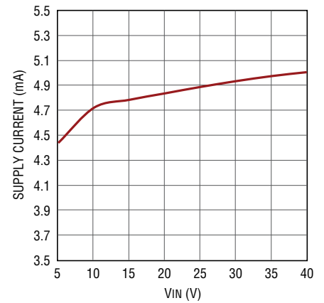
Quiescent Current vs Input Voltage without \text{EXTV}_{\text{CC}}
