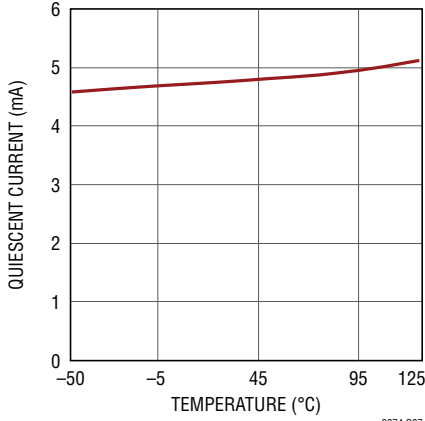
Quiescent Current vs Temperature without \text{EXTV}_{\text{CC}}
