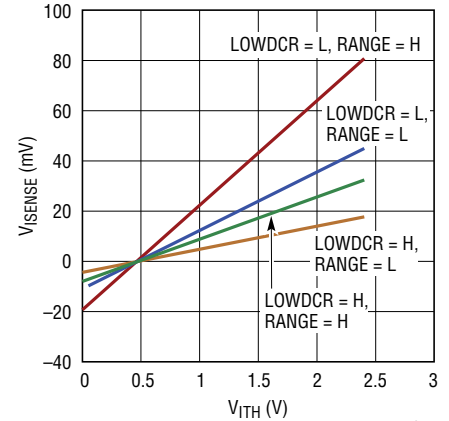
Current Sense Threshold vs I_{\text{TH}} Voltage
