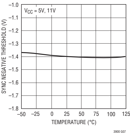
SYNC Negative Threshold vs Temperature
