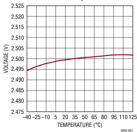
V_{\text{FLOAT}}(\text{CC/CV}) or, V_{\text{ABSORB}}(\text{Lead-Acid}) Reference vs Temperature
