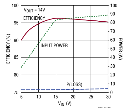
5V to 30V 6-Cell Lead-Acid Supply/Charger Maximum Power Efficiency vs V_{IN}
