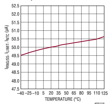
I_{RNG/SS} , I_{LIMIT} , I_{INTC} vs Temperature
