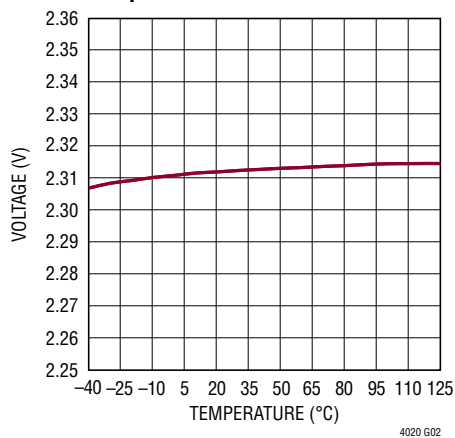
V_{\text{FLOAT}}(\text{Lead-Acid}) Reference vs Temperature
