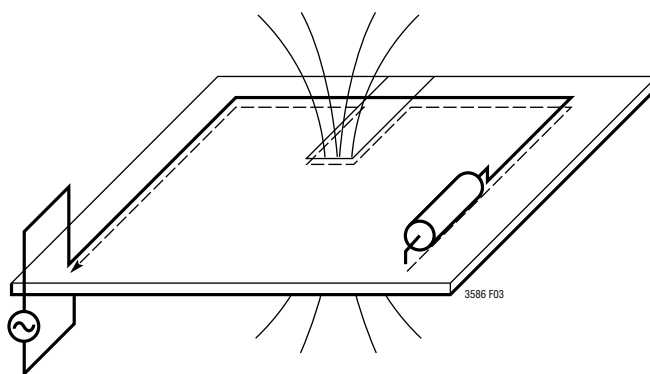
Figure 3. High Frequency Ground Currents Follow Their Incident Path. Slits in the Ground Plane Cause High Voltage and Increased EMI
