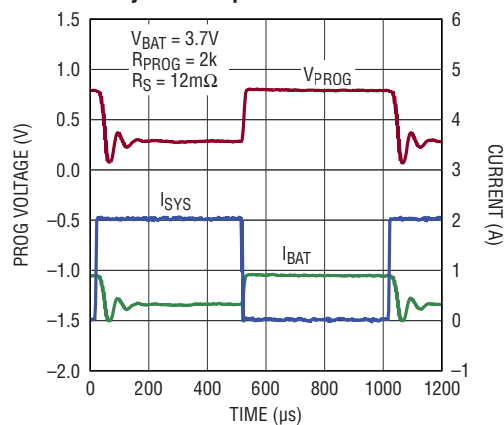
PROG Voltage Transient Response to System Step Load
