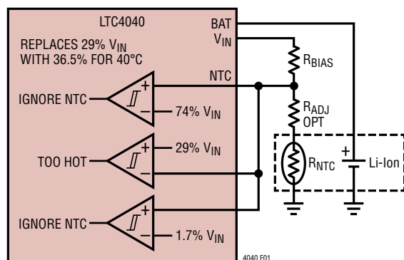
Figure 1. NTC Connections
