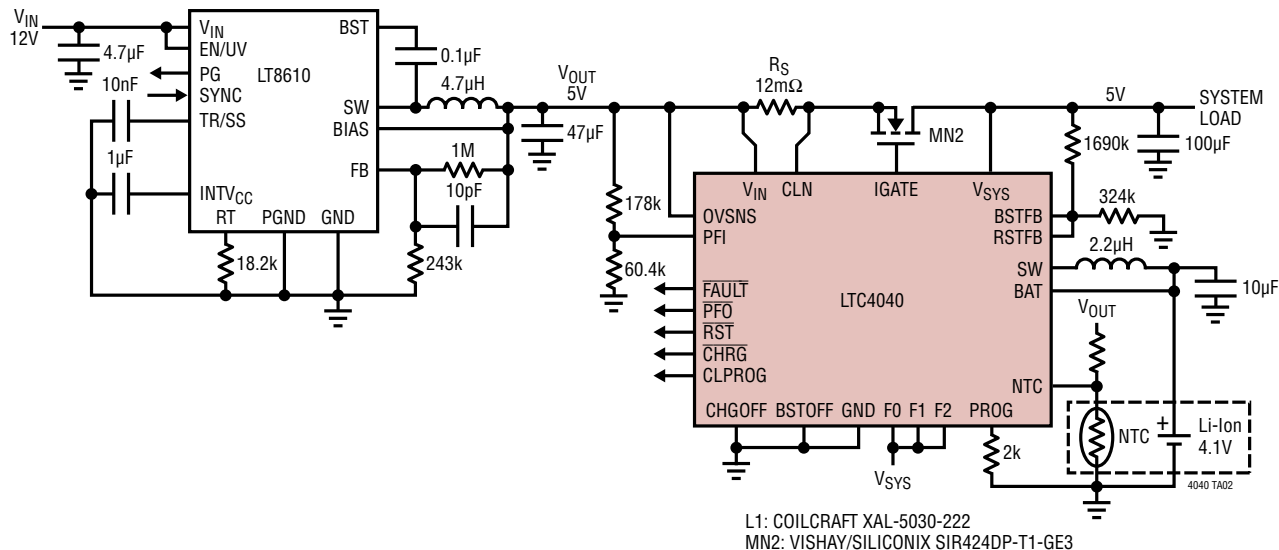
5V Backup System with 12V Buck for Automotive Application (Charge Current Setting: 1A, Input Current Limit Setting: 2A)
