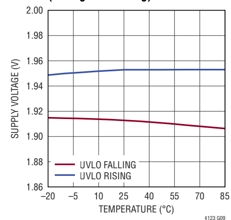
UVLO Threshold vs Temperature (Rising and Falling)
