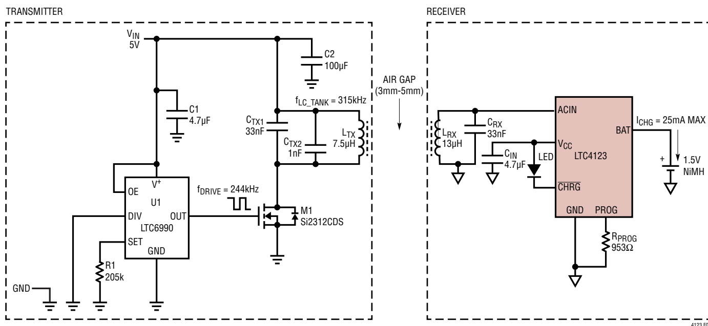
Figure 4. DC/AC Converter, Transmit/Receive Coils, Tuned Resonant LTC4123 Receiver
