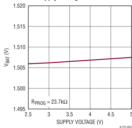
Battery Charge Voltage vs Supply Voltage
