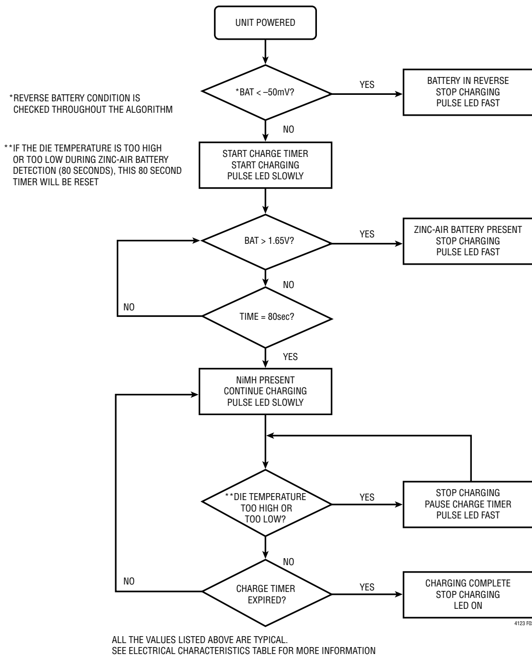
Figure 2. Charge Algorithm
