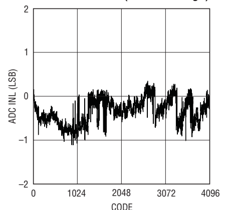
ADC INL vs Code (SENSE Voltage)
