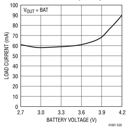
OTG Boost Burst Mode Current Threshold vs Battery Voltage
