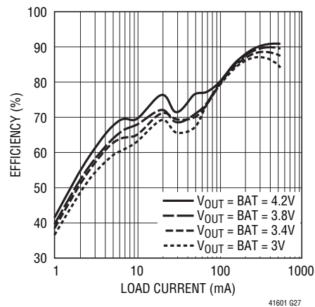
OTG Boost Efficiency vs Load Current
