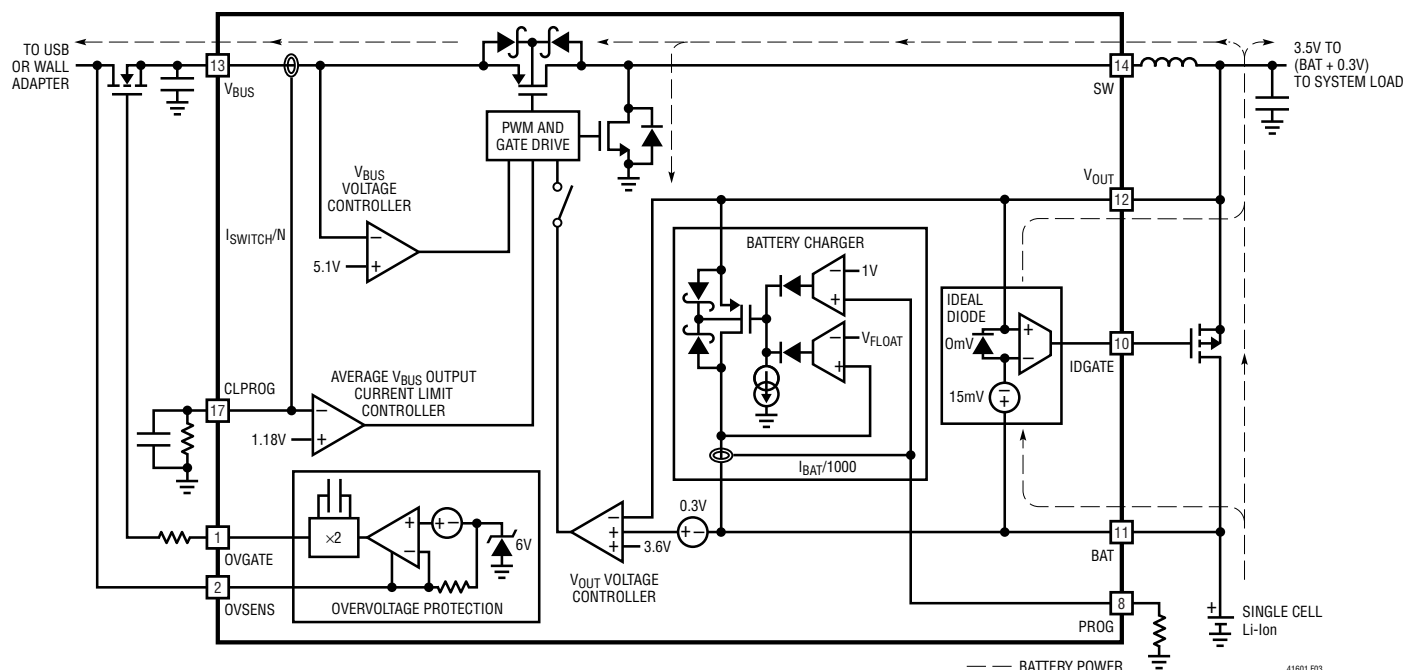
Figure 3. PowerPath Block Diagram – USB On-The-Go
