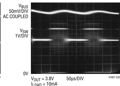
OTG Boost Burst Mode Operation
