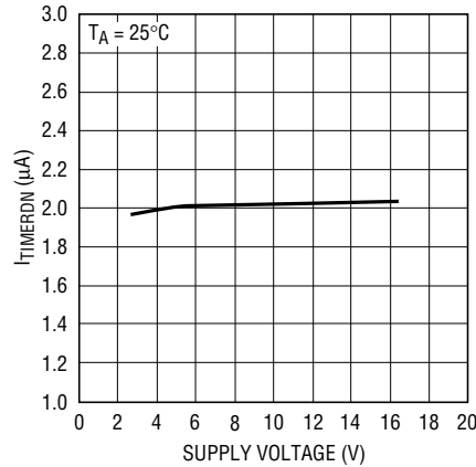
I_{TIMERDN} (In Cool-Off Cycle) vs Supply Voltage
