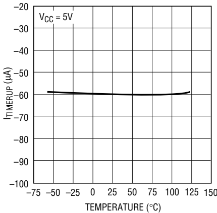
I_{TIMERUP} (During Circuit Breaker Delay) vs Temperature
