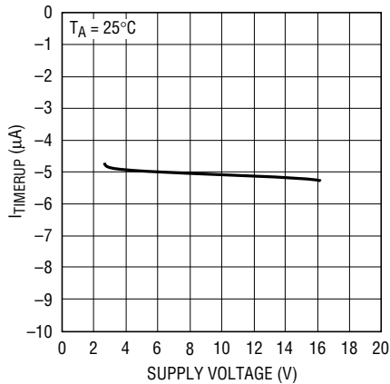
I_{TIMERUP} (In Initial Cycle) vs Supply Voltage
