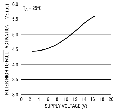
FILTER High to \overline{FAULT} Activation Time vs Supply Voltage
