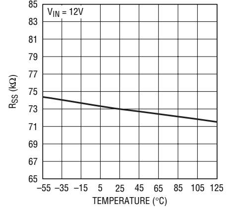
R_{SS} vs Temperature
