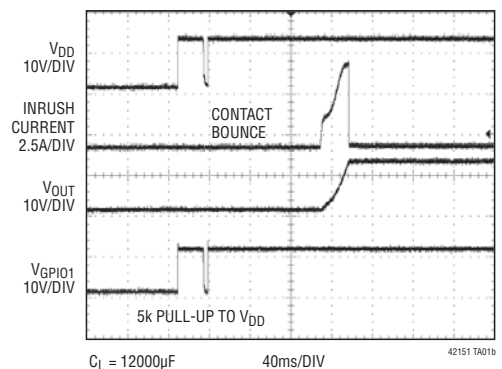
Start-Up Waveform
