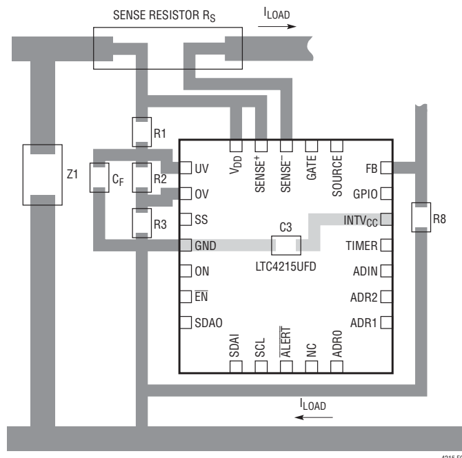
Figure 5. Recommended Layout
