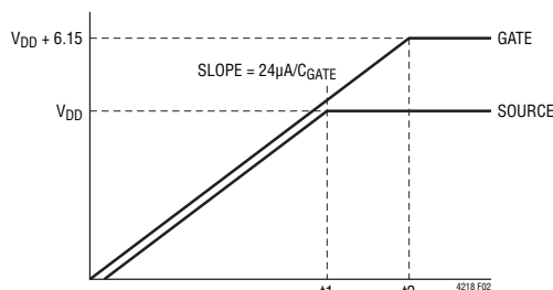
Figure 2. Supply Turn-On
