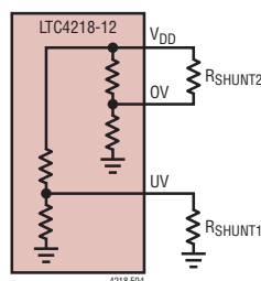
Figure 4. Adjusting LTC4218-12 Thresholds
