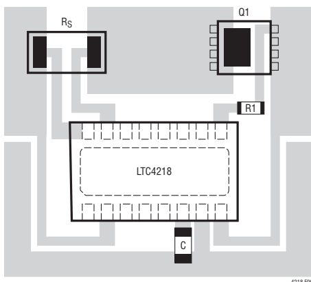
Figure 6. Recommended Layout
