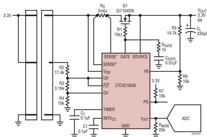
Figure 7. 3.3V, 6A Card Resident Application
