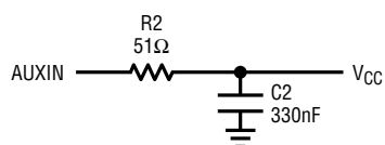
Figure 11. RC Network for V CC Filtering
