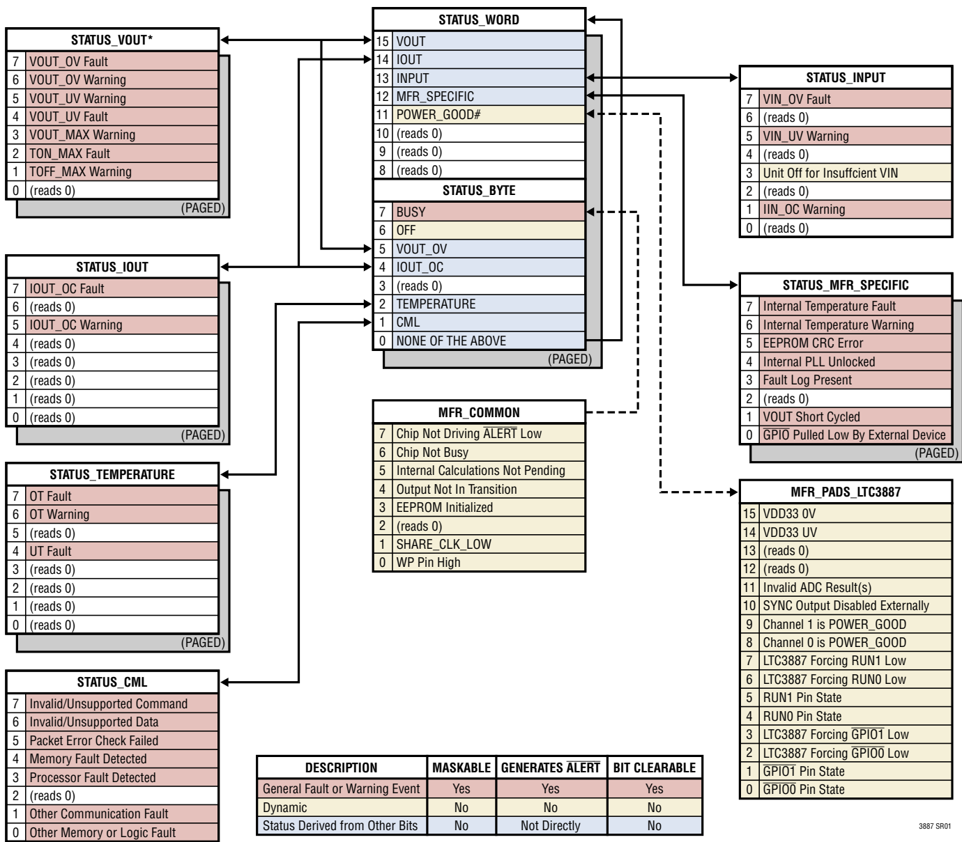
Figure 43. Summary of the Status Registers
