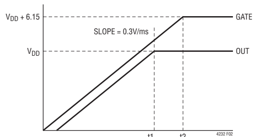
Figure 2. Supply Turn-On
