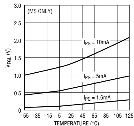
V_{PGL} vs Temperature
