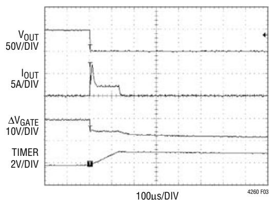
Figure 3. Short-Circuit Waveforms
