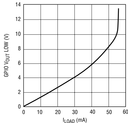
GPIO V_{\text{OUT Low}} vs I_{\text{LOAD}}
