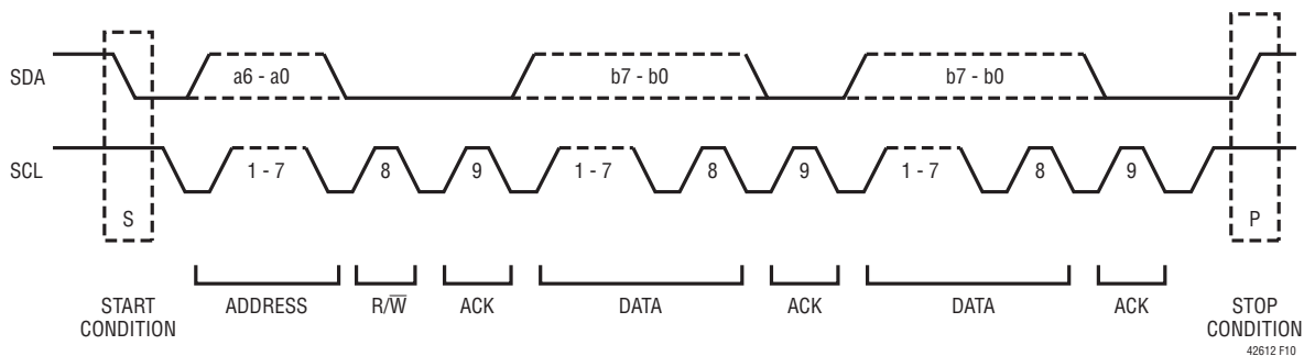
Figure 10. Data Transfer over I 2 C or SMBus
