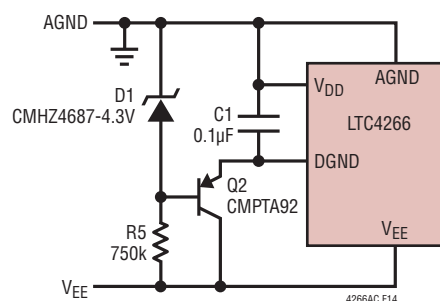
Figure 14. Negative LDO to DGND
