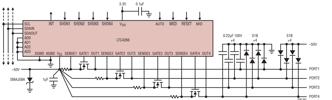
Complete 4-Port Ethernet High Power Source
