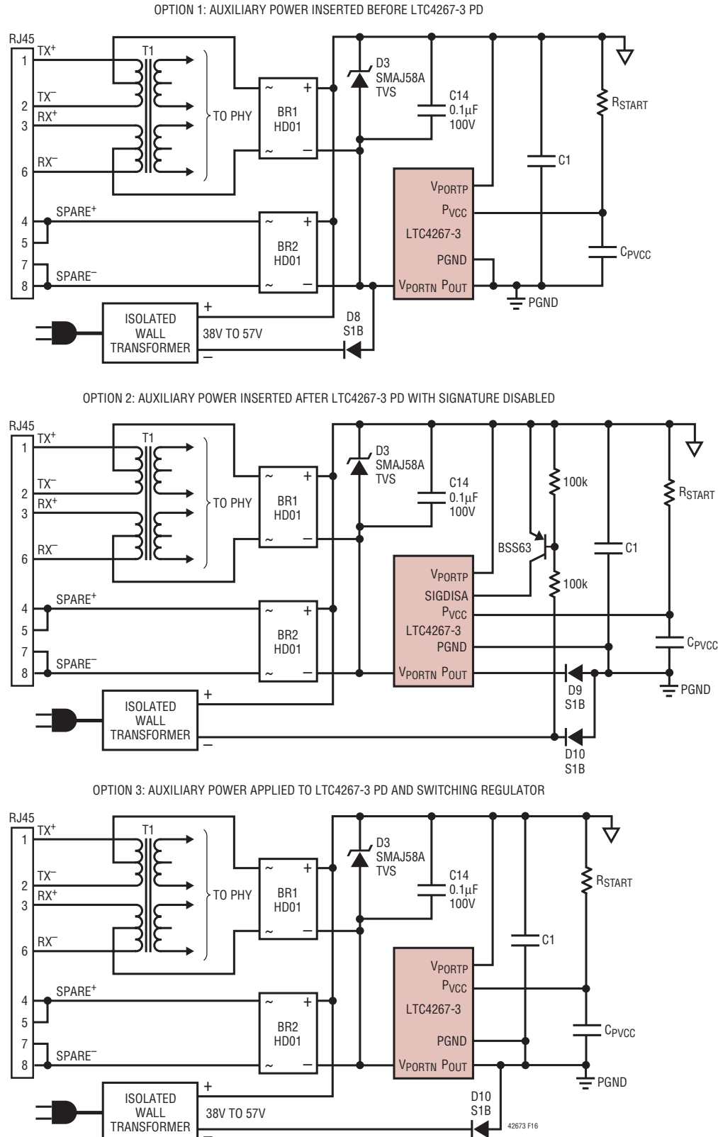
Figure 16. Auxiliary Power Source for PD
