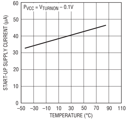
Start-Up I_{PVCC} Supply Current vs Temperature
