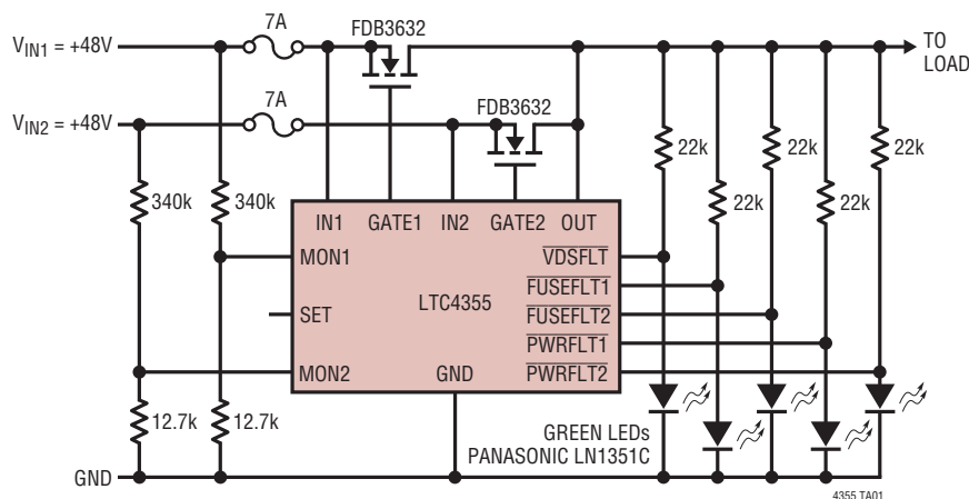
+48V Diode-OR
