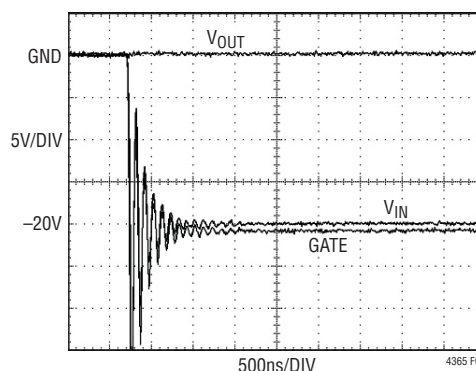
Figure 7. Hot Swapping V_{\text{IN}} to -20\text{V}
