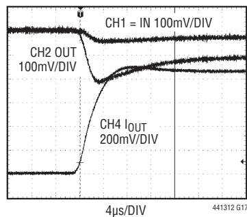
Response to 800mA Load Step in <16\mu s
