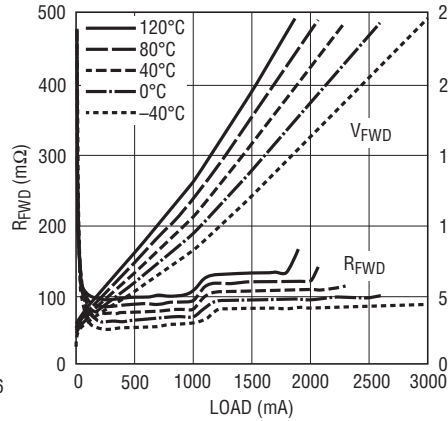
V_{FWD} and R_{FWD} vs I_{LOAD} (Linear)
