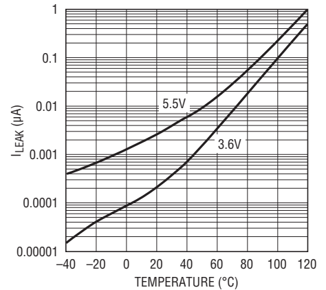
I_{LEAK} vs Temperature at V_{REVERSE} = 5.5V
