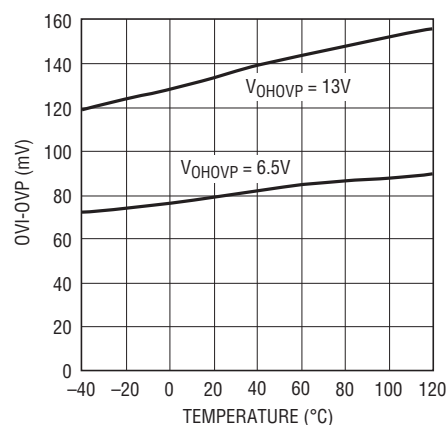
OVI-OVP vs Temperature (LTC4413-2 Only)
