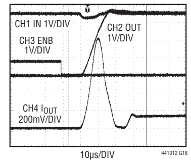
ENB Turn-On, 30 \mu s to Turn On with 180mA Load
