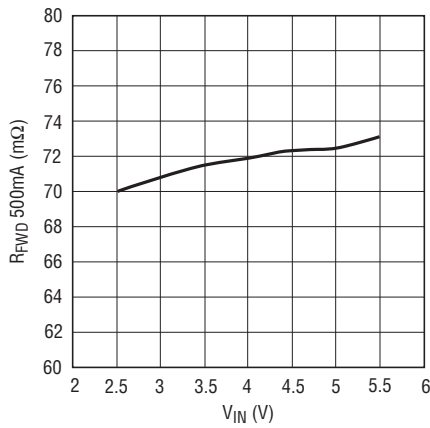
R_{FWD} vs V_{IN} and I_{LOAD} = 500mA
