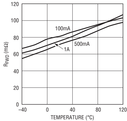
R_{FWD} vs Temperature
