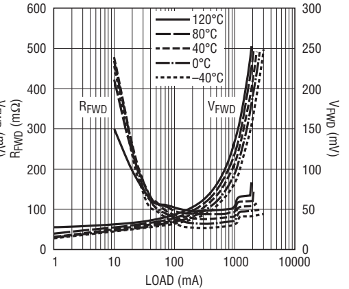
R_{FWD} and V_{FWD} vs I_{LOAD} (Log)
