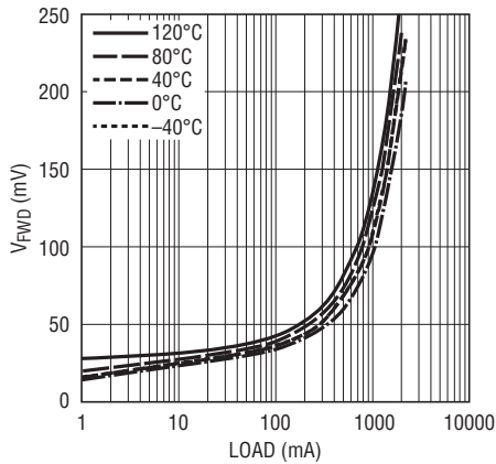
V_{FWD} vs I_{LOAD} (Log)
