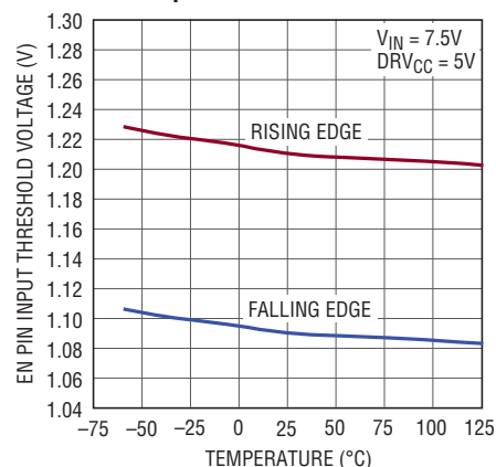
EN Pin Input Threshold Voltage vs Temperature
