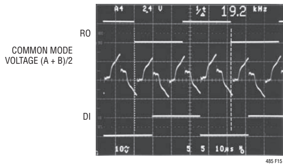
Figure 15. System Common Mode Voltage at 19.2kHz
