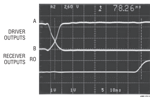
Figure 11. Receiver t_{PHL}
