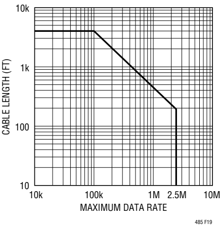
Figure 19. Cable Length vs Maximum Data Rate
