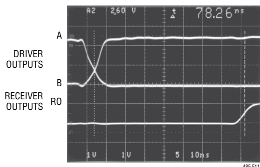
Figure 11. Receiver t_{PHL}
