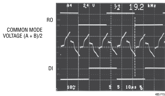
Figure 15. System Common Mode Voltage at 19.2kHz
