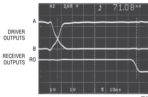
Figure 12. Receiver t_{PLH}
