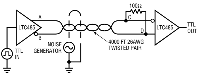
Figure 14. Line Length Test Circuit
