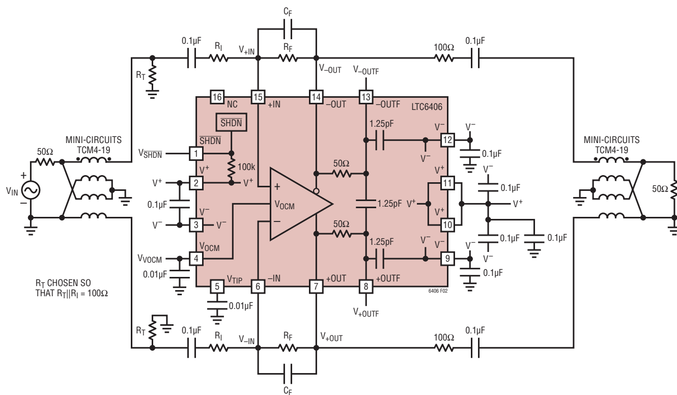
Figure 2. AC Test Circuit (–3dB BW Testing)
