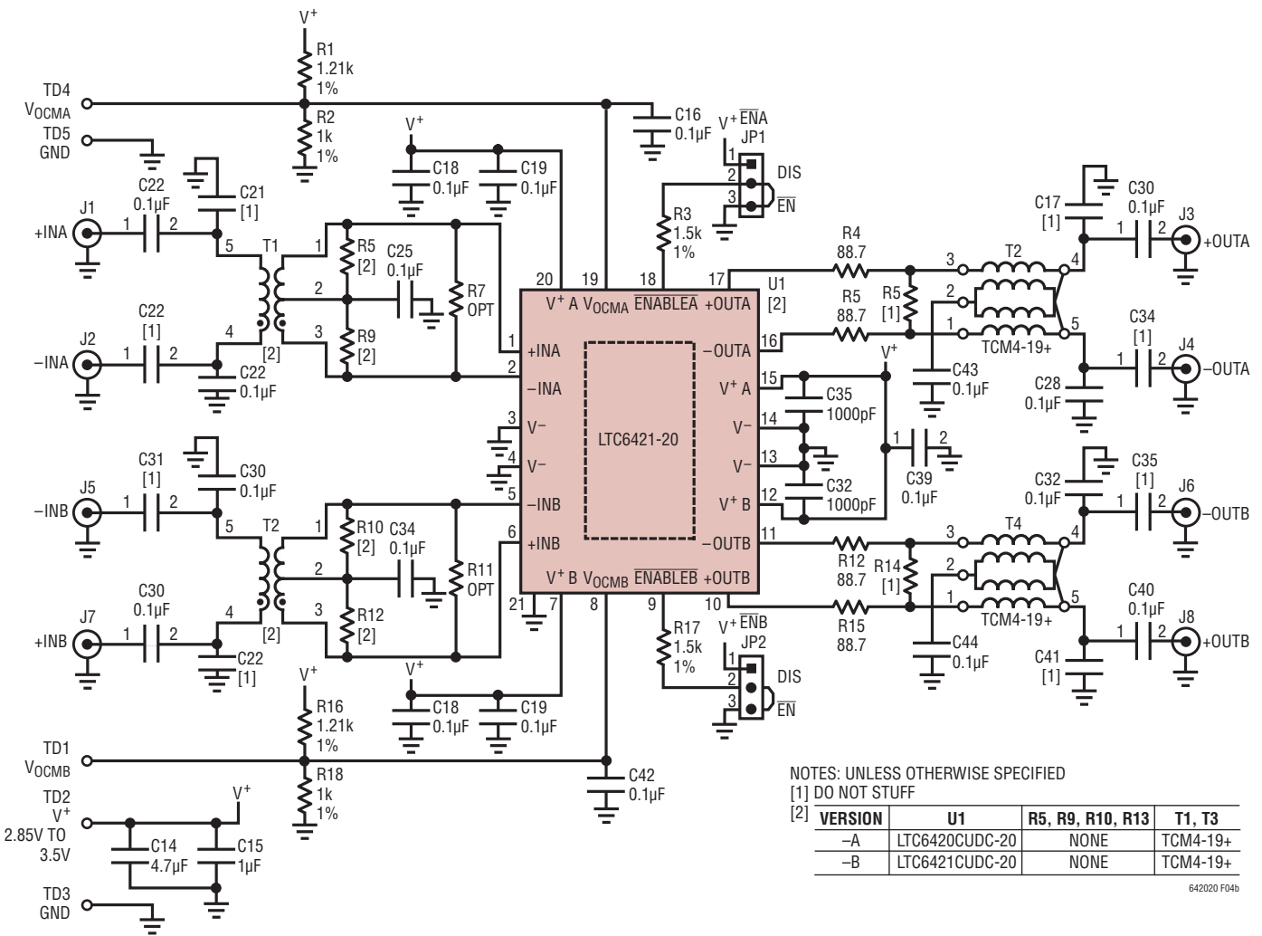
Figure 4b. Demo Circuit 1299 Schematic (Test Circuit A)
