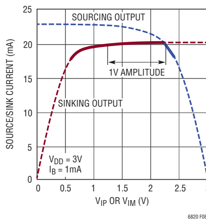
Figure 8. Drive Source/Sink vs Output Voltage
