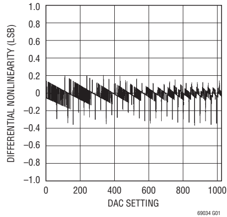
Differential Nonlinearity
