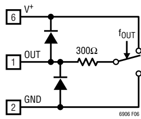
Figure 6. OUT Pin
