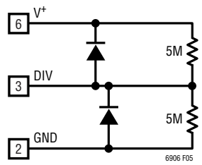
Figure 5. DIV Pin
