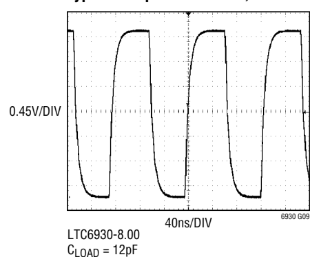
Typical Output Waveform, 8MHz
