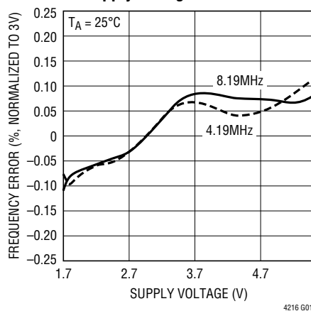
Typical Frequency Error vs Supply Voltage
