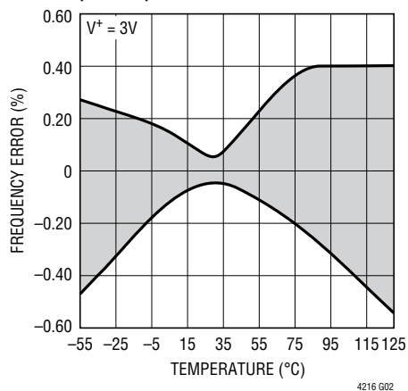
Typical Frequency Error vs Temperature, MS8 Package (Note 3)
