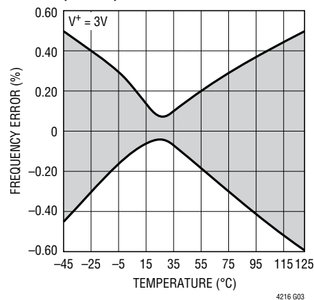
Typical Frequency Error vs Temperature, DFN Package (Note 3)
