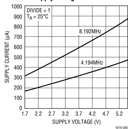
Typical Supply Current vs Supply Voltage
