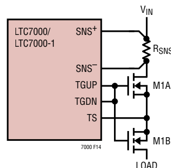
Figure 14. Protecting Load from Voltage Drops on V_{IN}
