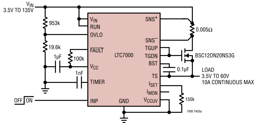
High Side Switch with Input Overvoltage and Overcurrent Protection
