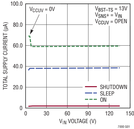
Total Supply Current vs V_{IN} Voltage
