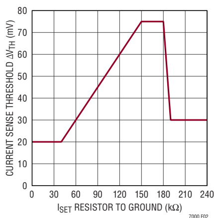
Figure 2. R_{ISET} Selection
