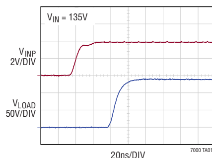
Turn-On Transient Waveform
