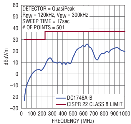
Figure 17. Low EMI Demo Board Emissions
