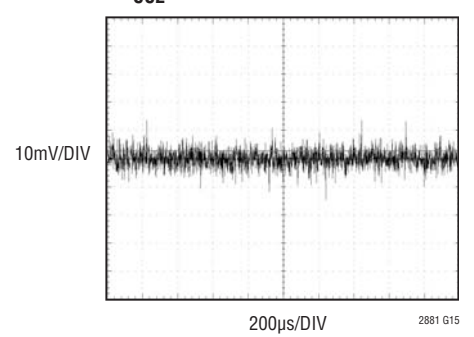
V_{CC2} Noise
