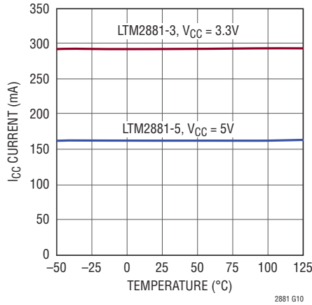
V_{CC} Supply Current vs Temperature at I_{LOAD} = 100mA on V_{CC2}
