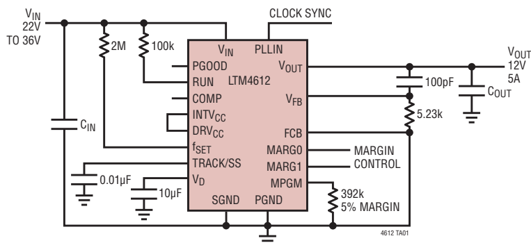
12V/5A Ultralow Noise \mu Module with 22V to 36V Input
