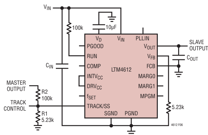
Figure 6. Coincident Tracking
