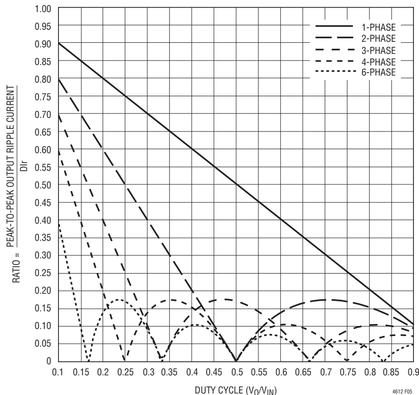
Figure 5. Normalized Output Ripple Current vs Duty Cycle, DI_L = V_0 T / L_I
