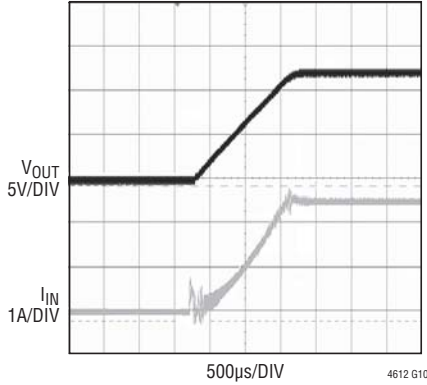
Start-Up with 24V_{IN} to 12V_{OUT} at I_{OUT} = 5A , T_A = -55^\circ C
