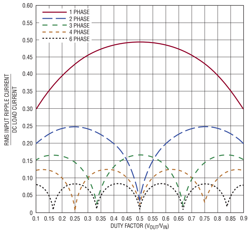
Figure 2. Normalized Input RMS Ripple Current vs Duty Factor for One to Six \mu Module Regulators (Phases)
