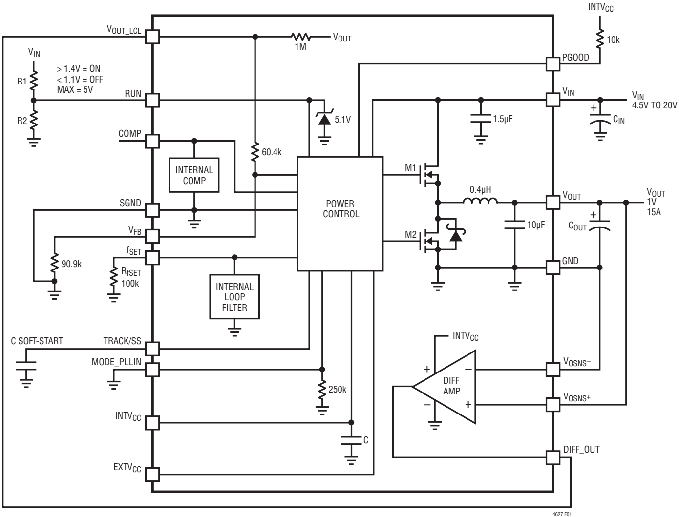
Figure 1. Simplified LTM4627 Block Diagram
