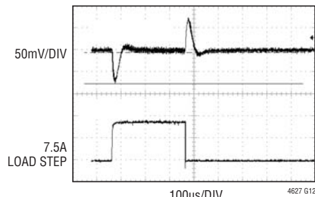
5.0V Transient Response
