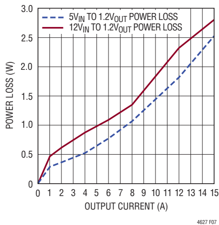
Figure 7. 1.2V OUT Power Loss
