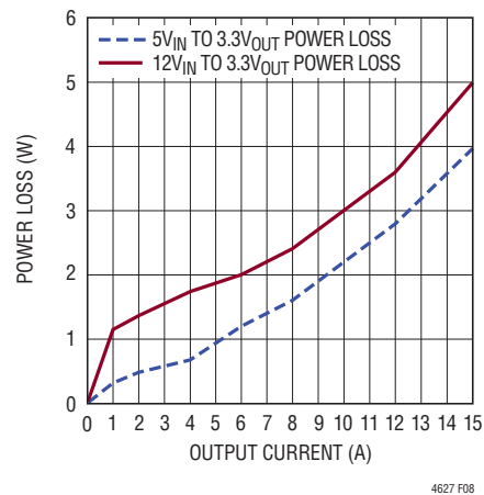
Figure 8. 3.3V OUT Power Loss
