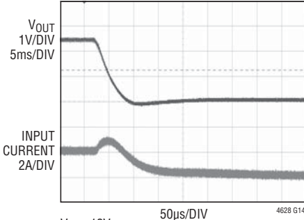
Output Short-Circuit
