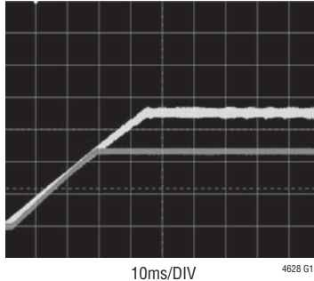
Coincident Tracking
