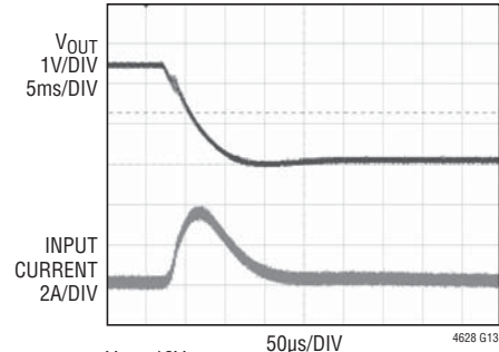
Output Short-Circuit
