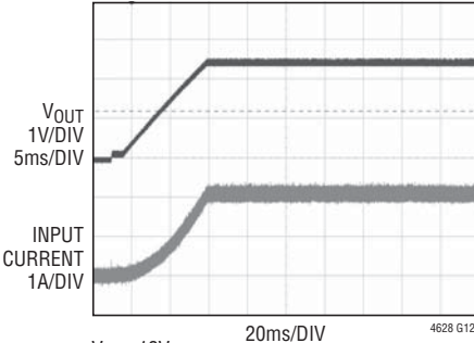
Output Start-Up
