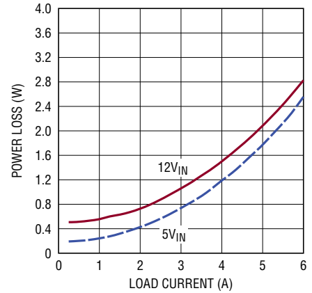
Figure 11. 2.5V Output Power Loss
