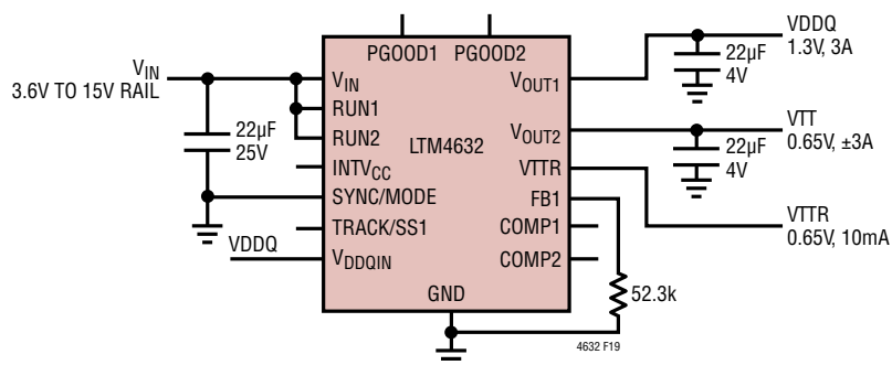
Figure 19. 3.6V to 15V Input, 1.5V/3A VDDQ, 0.75V/ \pm 3A VTT and 10mA VTTR Design
