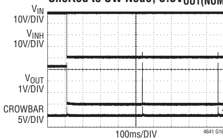
Autonomous Restart with V_{INH} Shorted to SW Node, 3.3V_{OUT(NOM)}
