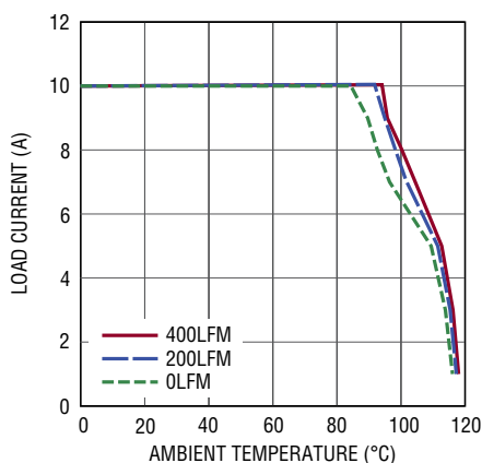
Figure 14. No Heat Sink with 5V IN to 2.5V OUT
