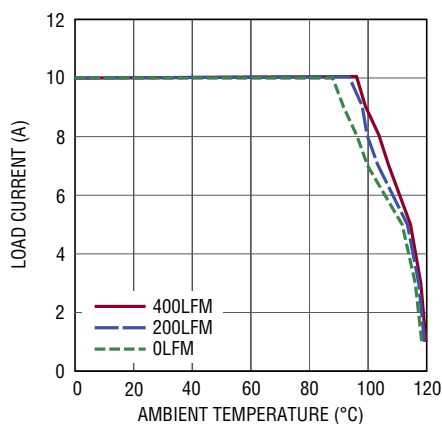
Figure 12. No Heat Sink with 5V IN to 1.5V OUT
