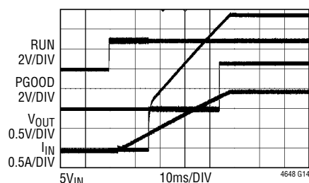
Output Start-Up
