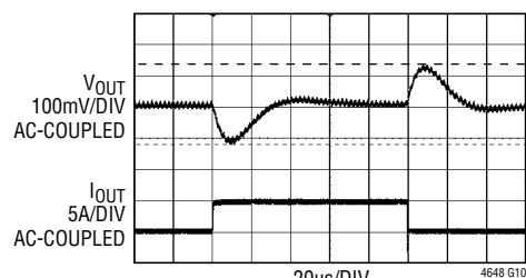
3.3V IN , 2.5V OUT Load Transient
