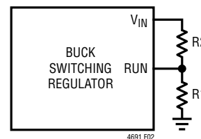
Figure 2. RUN Divider
