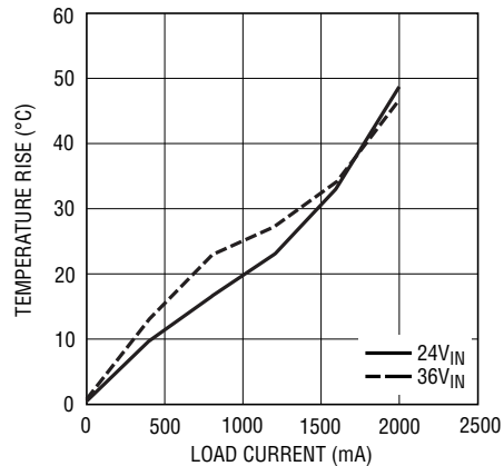
Temperature Rise vs Load Current, V_{OUT} = 10\text{V} (BGA)
