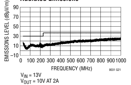
Radiated Emissions
