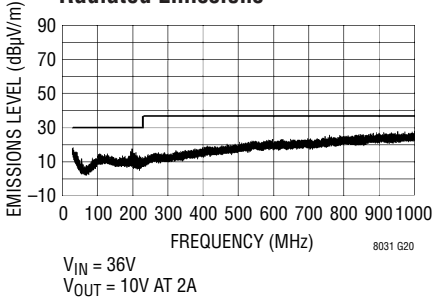
Radiated Emissions
