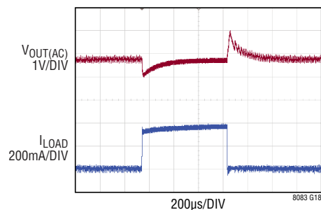
Transient Response from 36V_{IN} to 36V_{OUT}
