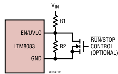
Figure 4. V IN Undervoltage Lockout (UVLO)
