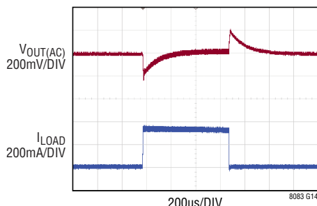
Transient Response from 12V_{IN} to 12V_{OUT}
