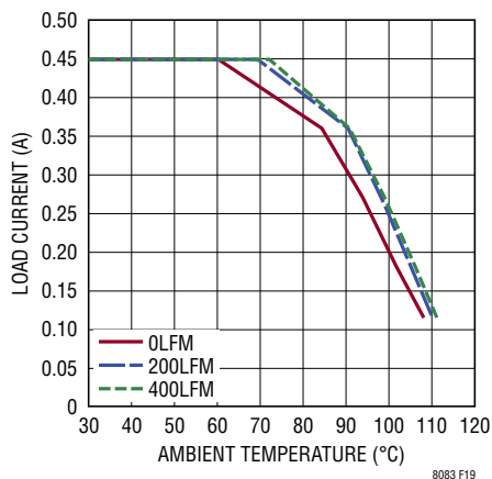
Figure 19. 12V to 36V Derating Curve, No Heat Sink
