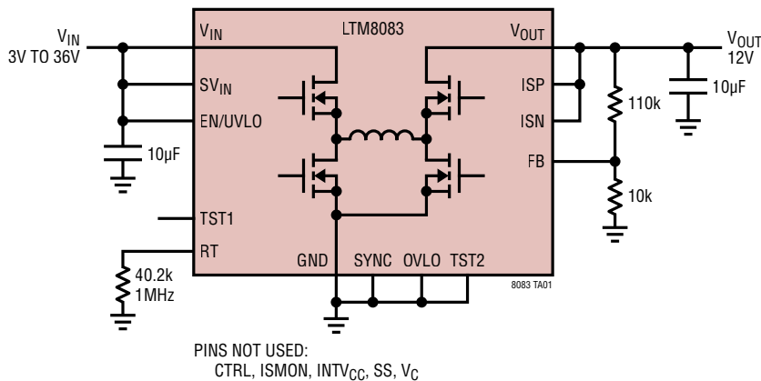
12V OUT from 3-36V IN Buck-Boost Regulator
