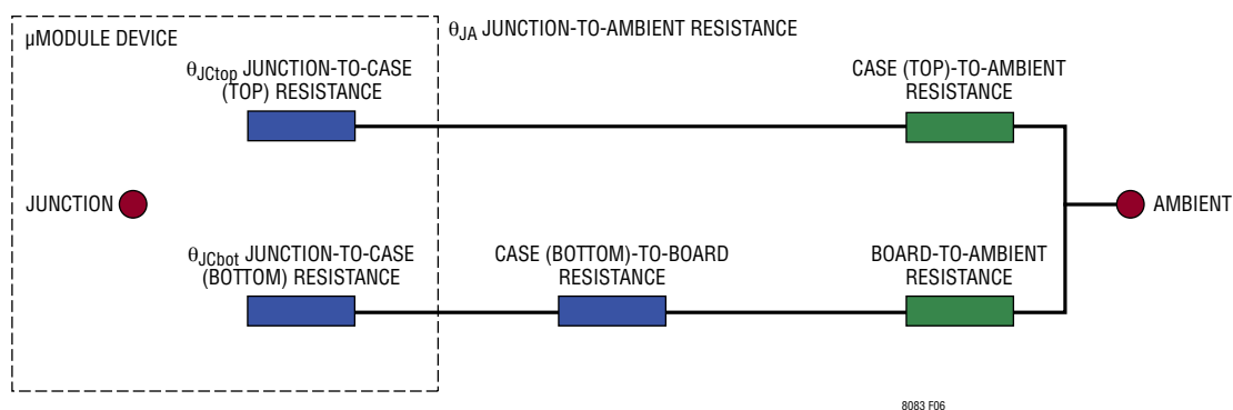
Figure 6. Graphical Approximation of the Thermal Coefficients, Including JESD 51-12 Terms
