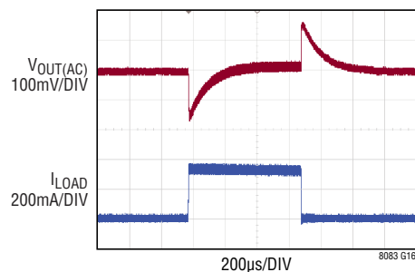
Transient Response from 36V_{IN} to 12V_{OUT}
