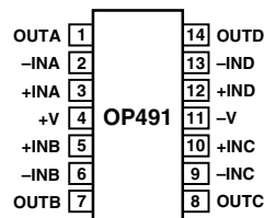
14-Lead SO
