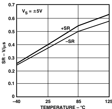
TPC 50. Slew Rate vs. Temperature, V_S = \pm 5\text{ V}
