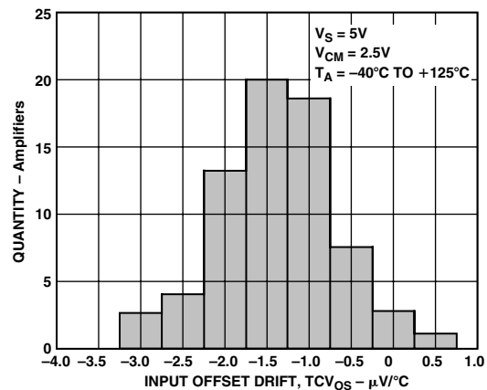
TPC 4. Input Offset Voltage Distribution (TCV 0s )
