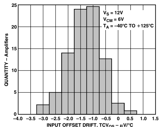
TPC 5. Input Offset Voltage Distribution (TCV 0s )
