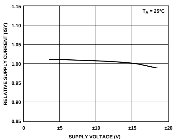
Figure 33. OP482 Relative Supply Current vs. Supply Voltage
