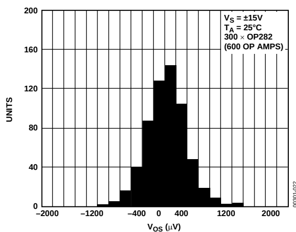
Figure 22. OP282 V_{OS} Distribution SOIC Package
