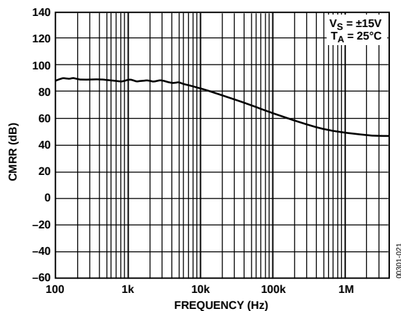
Figure 21. OP282 CMRR vs. Frequency
