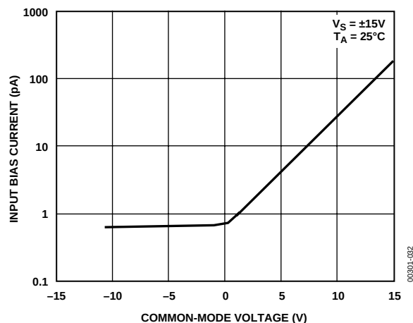
Figure 32. OP482 Input Bias Current vs. Common-Mode Voltage
