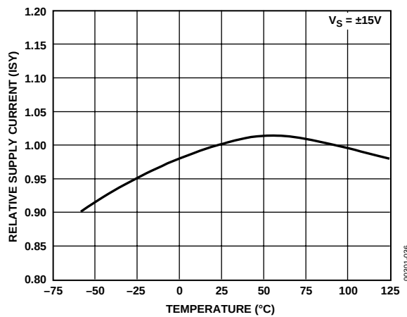
Figure 36. OP482 Relative Supply Current vs. Temperature
