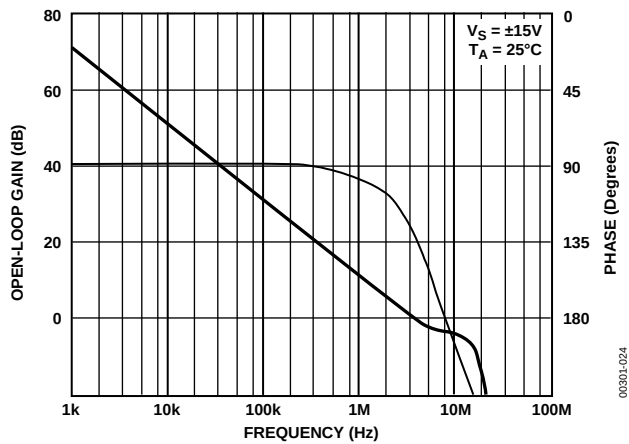
Figure 24. OP482 Open-Loop Gain, Phase vs. Frequency
