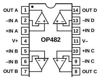
Figure 3. 14-Lead PDIP (P-Suffix) [N-14]
