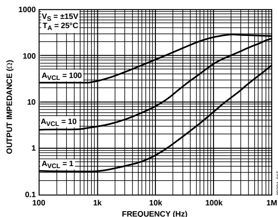
Figure 15. OP282 Closed-Loop Output Impedance vs. Frequency
