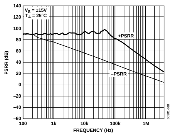
Figure 18. OP282 PSRR vs. Frequency
