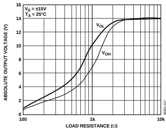
Figure 17. OP282 Absolute Output Voltage vs. Load Resistance
