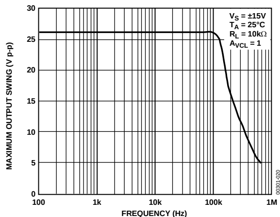
Figure 20. OP282 Maximum Output Swing vs. Frequency
