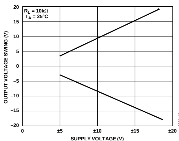
Figure 34. OP482 Output Voltage Swing vs. Supply Voltage
