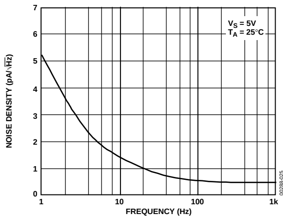
Figure 24. Current Noise Density vs. Frequency
