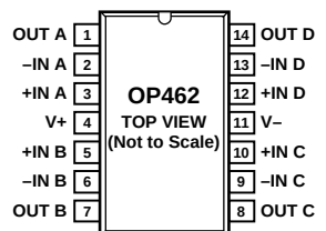
Figure 4. 14-Lead Narrow-Body SOIC (S Suffix)
