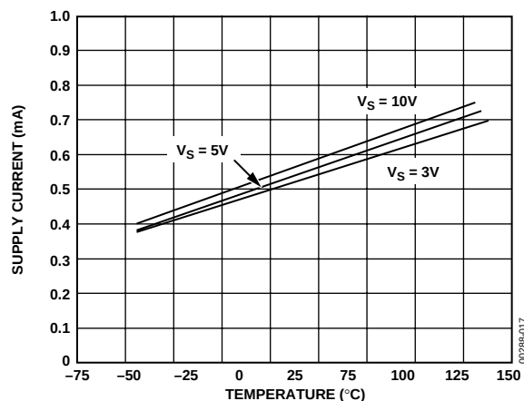
Figure 16. Supply Current/Amplifier vs. Temperature
