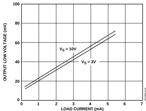
Figure 15. Output Low Voltage to Supply Rail vs. Load Current
