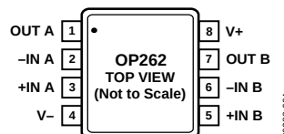
Figure 3. 8-Lead TSSOP (RU Suffix)
