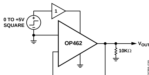
Figure 38. Test Circuit for Power-On Settling Time
