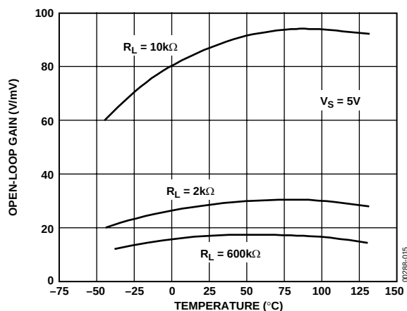
Figure 14. OP462 Open-Loop Gain vs. Temperature
