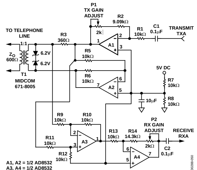
Figure 49. Single-Supply Direct Access Arrangement for Modems
