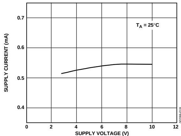
Figure 17. OP462 Supply Current/Amplifier vs. Supply Voltage
