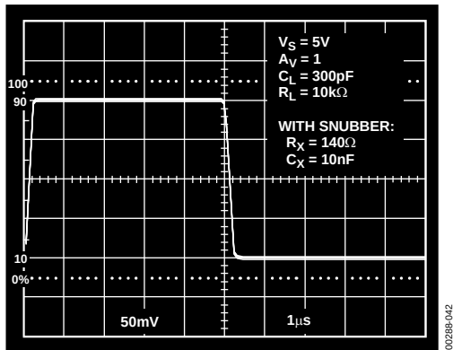
Figure 41. A Photo of a Nice Square Wave at the Output
