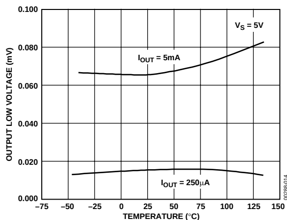
Figure 13. OP462 Output Low Voltage vs. Temperature
