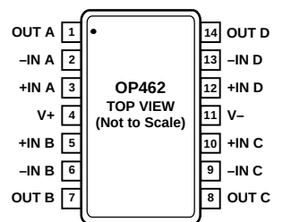
Figure 5. 14-Lead TSSOP (RU Suffix)
