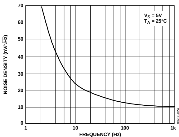
Figure 23. Voltage Noise Density vs. Frequency
