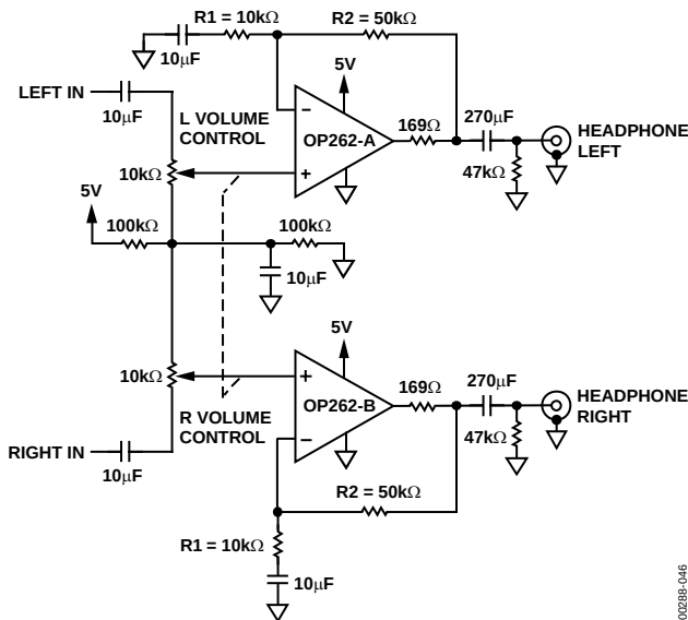
Figure 45. Headphone Output Amplifier
