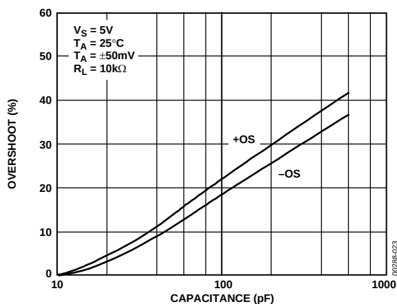
Figure 22. Small-Signal Overshoot vs. Capacitance
