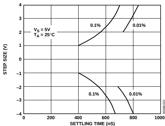
Figure 21. Step Size vs. Settling Time
