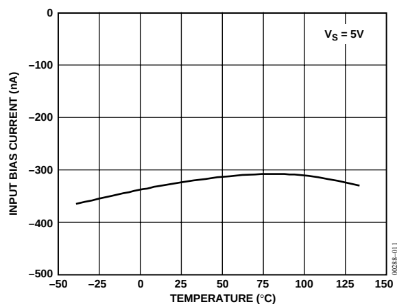
Figure 10. OP462 Input Bias Current vs. Temperature
