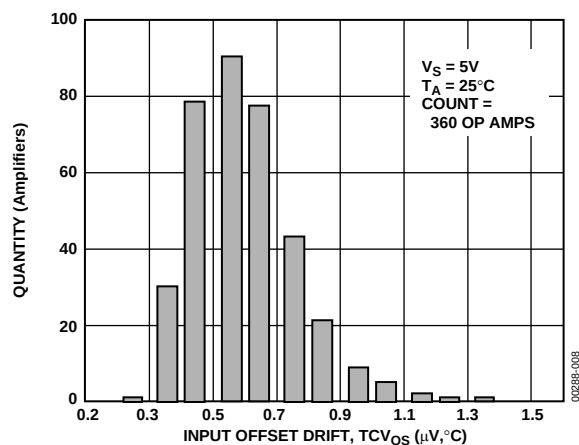
Figure 7. OP462 Input Offset Voltage Drift ( \text{TCV}_{OS} )
