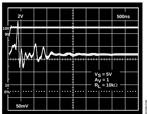
Figure 37. Oscilloscope Photo of V_S and V_{OUT}
