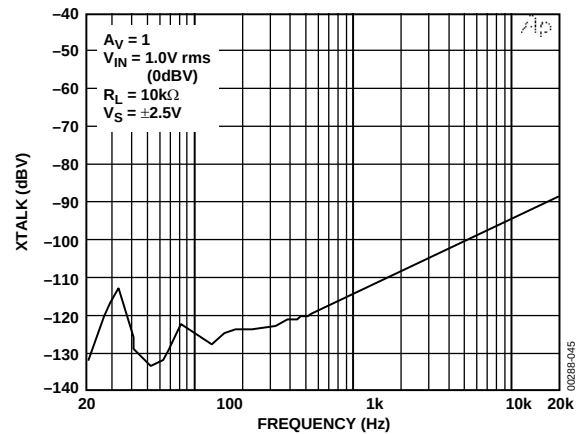
Figure 44. Crosstalk vs. Frequency
