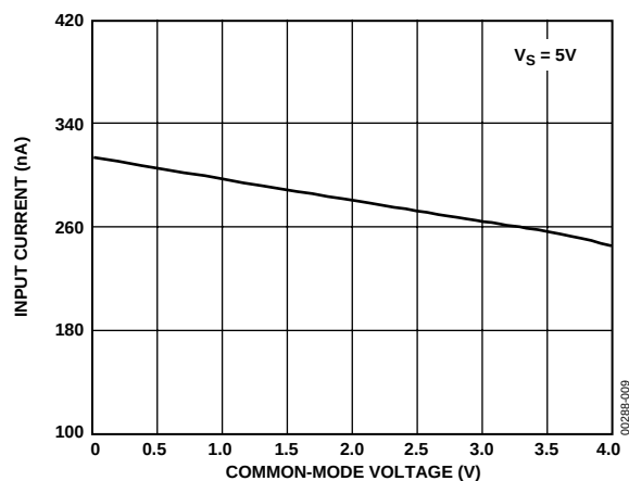
Figure 8. OP462 Input Bias Current vs. Common-Mode Voltage
