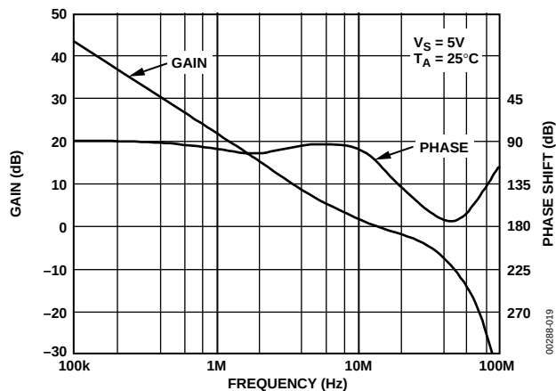
Figure 18. Open-Loop Gain and Phase vs. Frequency (No Load)
