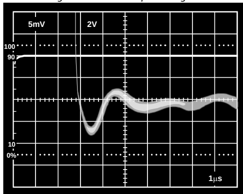
Figure 48. Negative Slope Settling Time
