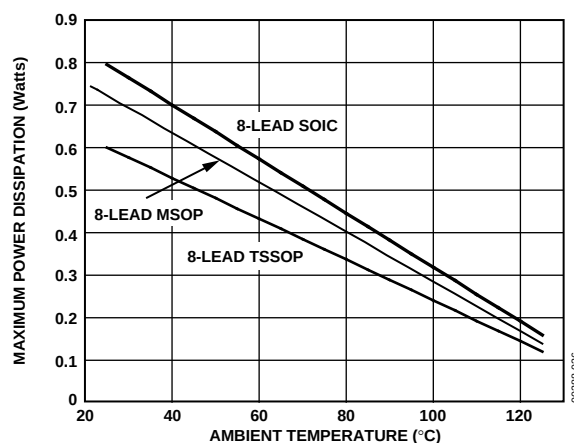
Figure 35. Maximum Power Dissipation vs. Temperature for 8-Lead Package Types
