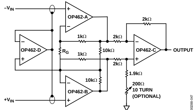
Figure 46. High Speed Instrumentation Amplifier
