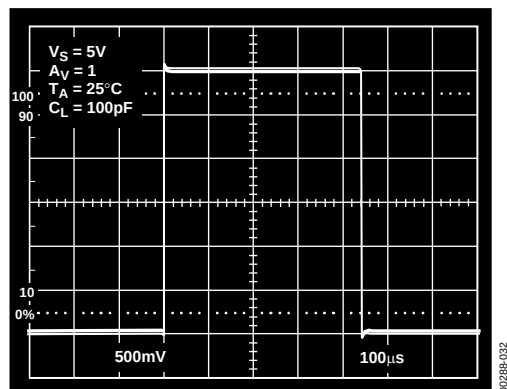
Figure 31. Large Signal Transient Response
