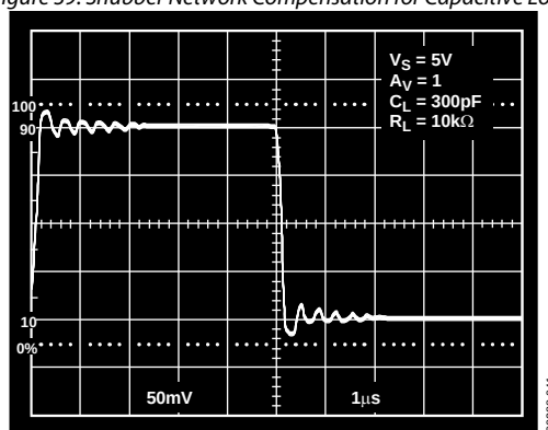
Figure 40. A Photo of a Ringing Square Wave
