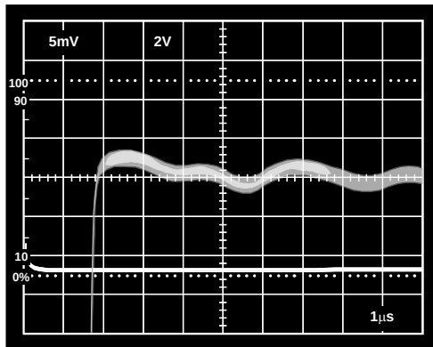
Figure 47. Positive Slope Settling Time
