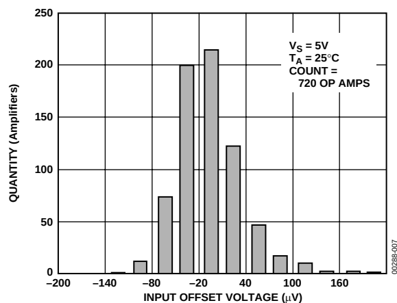
Figure 6. OP462 Input Offset Voltage Distribution
