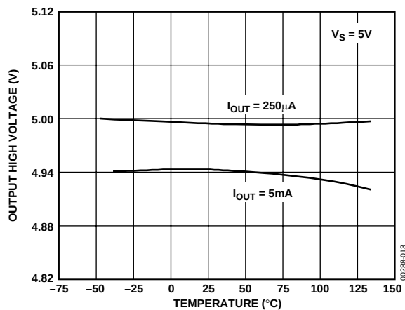
Figure 12. OP462 Output High Voltage vs. Temperature
