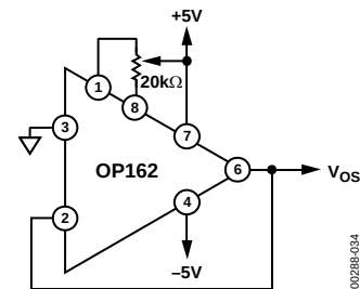
Figure 33. Offset Adjustment Schematic
