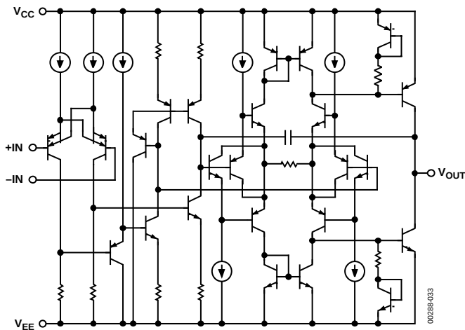
Figure 32. Simplified Schematic
