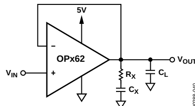
Figure 39. Snubber Network Compensation for Capacitive Loads
