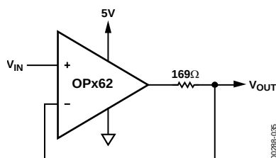
Figure 34. Output Short-Circuit Protection
