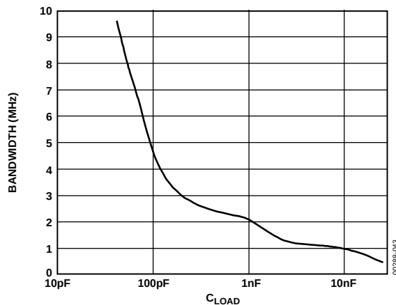
Figure 42. Unity-Gain Bandwidth vs. C_{LOAD}
