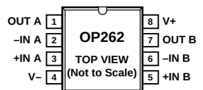
Figure 2. 8-Lead Narrow-Body SOIC (S Suffix)
