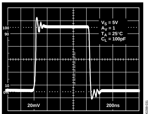
Figure 30. Small Signal Transient Response
