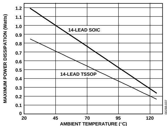
Figure 36. Maximum Power Dissipation vs. Temperature for 14-Lead Package Types
