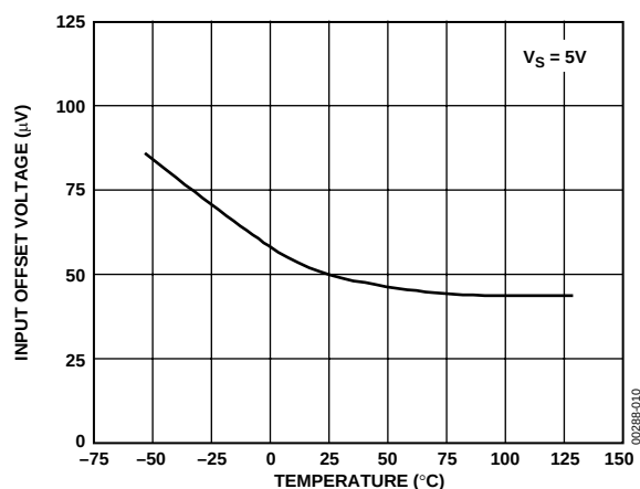
Figure 9. OP462 Input Offset Voltage vs. Temperature
