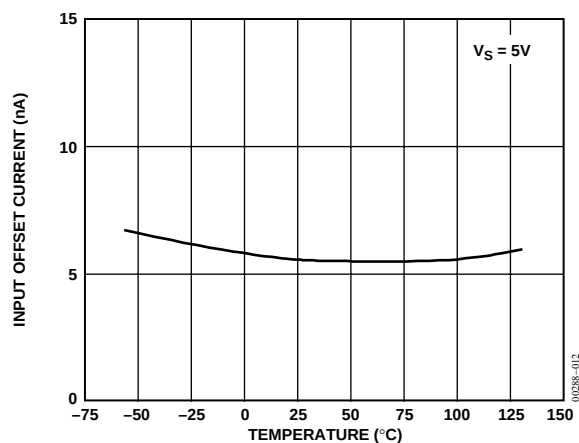
Figure 11. OP462 Input Offset Current vs. Temperature
