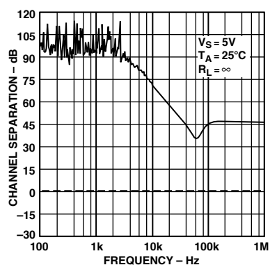
TPC 31. Channel Separation vs. Frequency
