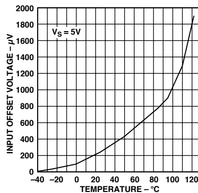
TPC 3. Input Offset Voltage vs. Temperature
