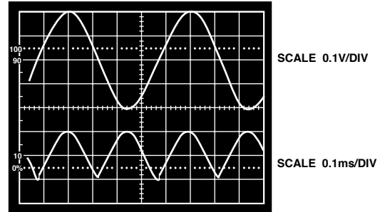
Figure 9. Full-Wave Rectified Signal
