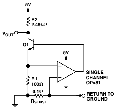
Figure 7. Low-Side Load Current Monitor
