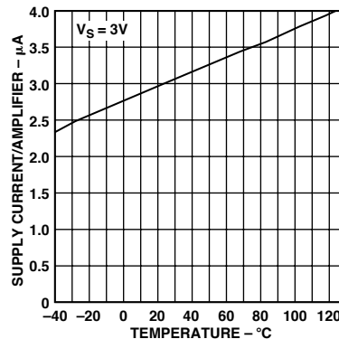
TPC 21. Supply Current/Amplifier vs. Temperature
