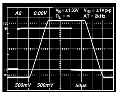
TPC 29. Saturation Recovery Time
