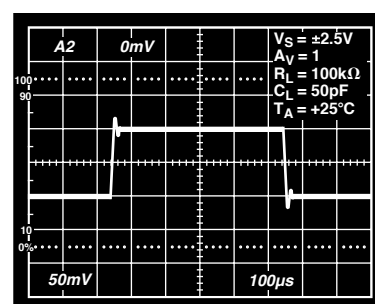
TPC 24. Small Signal Transient Response
