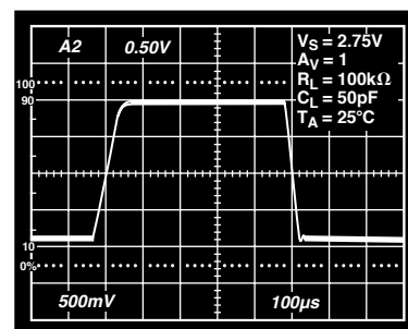
TPC 27. Large Signal Transient Response
