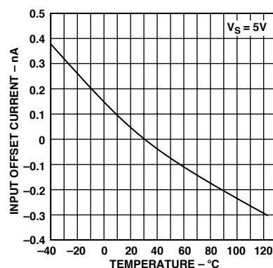
TPC 6. Input Offset Current vs. Temperature
